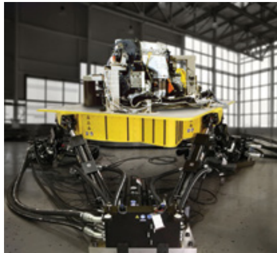
Model 354 Hexapod MAST System
